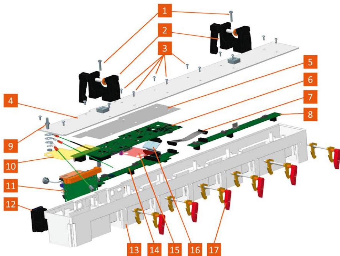
Figure 8 Exploded view 1 - M docking station
