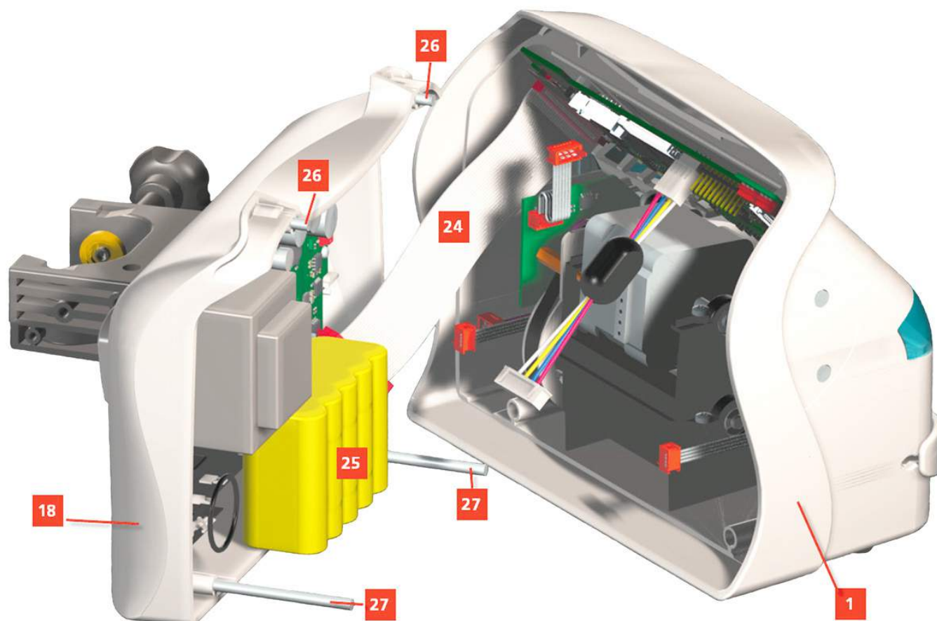
Figure 7 Exploded view, complete
