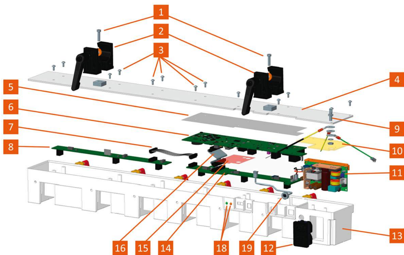
Figure 9 Exploded view 2 - M docking station
