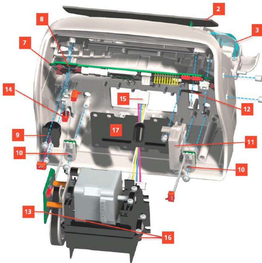
Figure 6 Casing backside, inside
