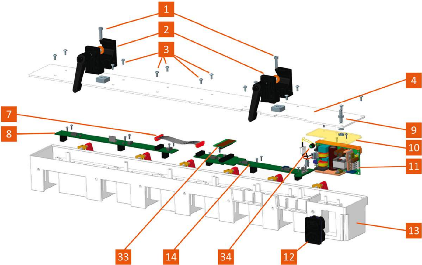
Figure 10 Exploded view - P docking station
