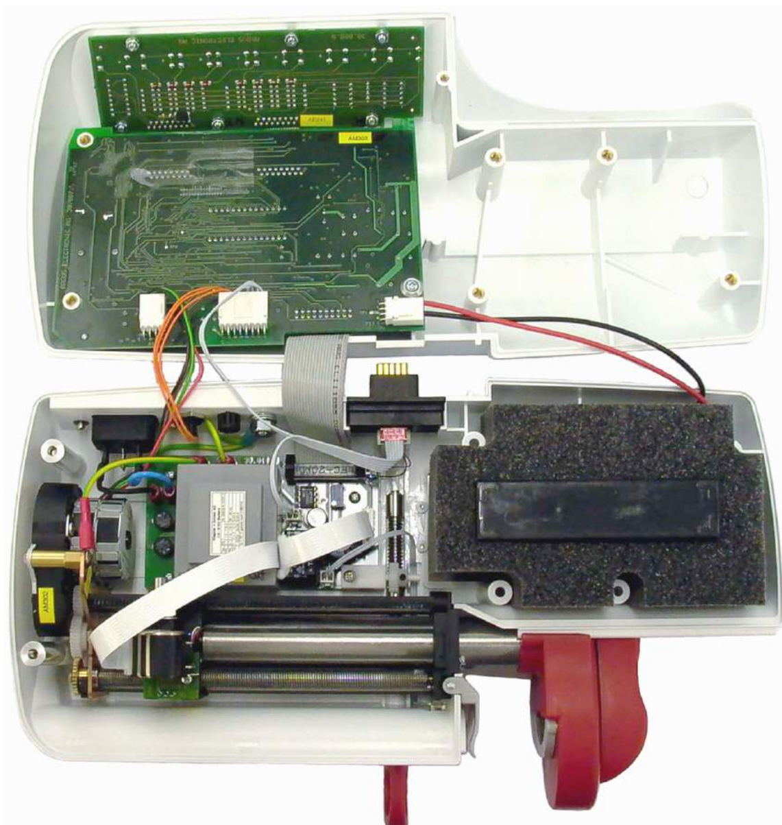
Figure 1 A600S - Opened view, complete
