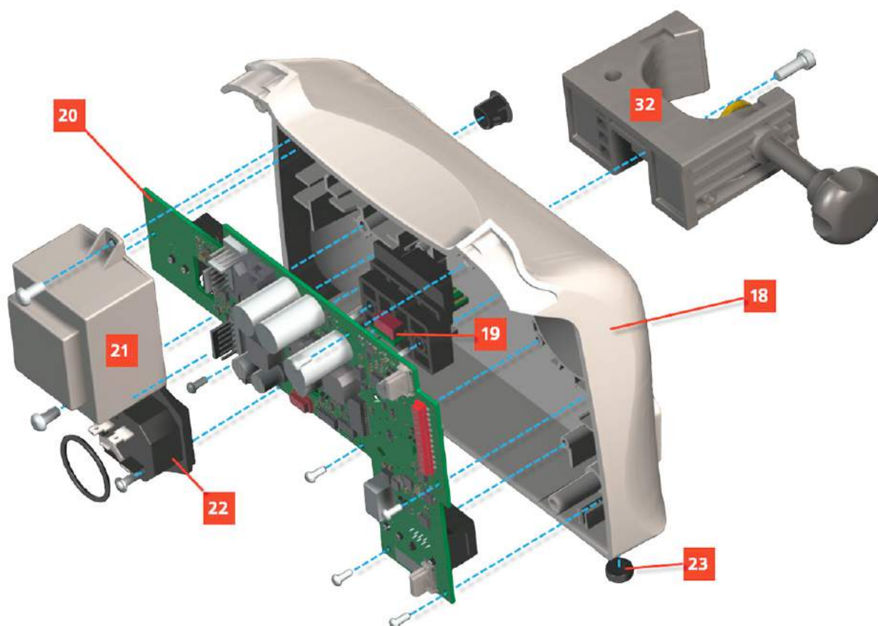
Figure 4 Casing front, inside
