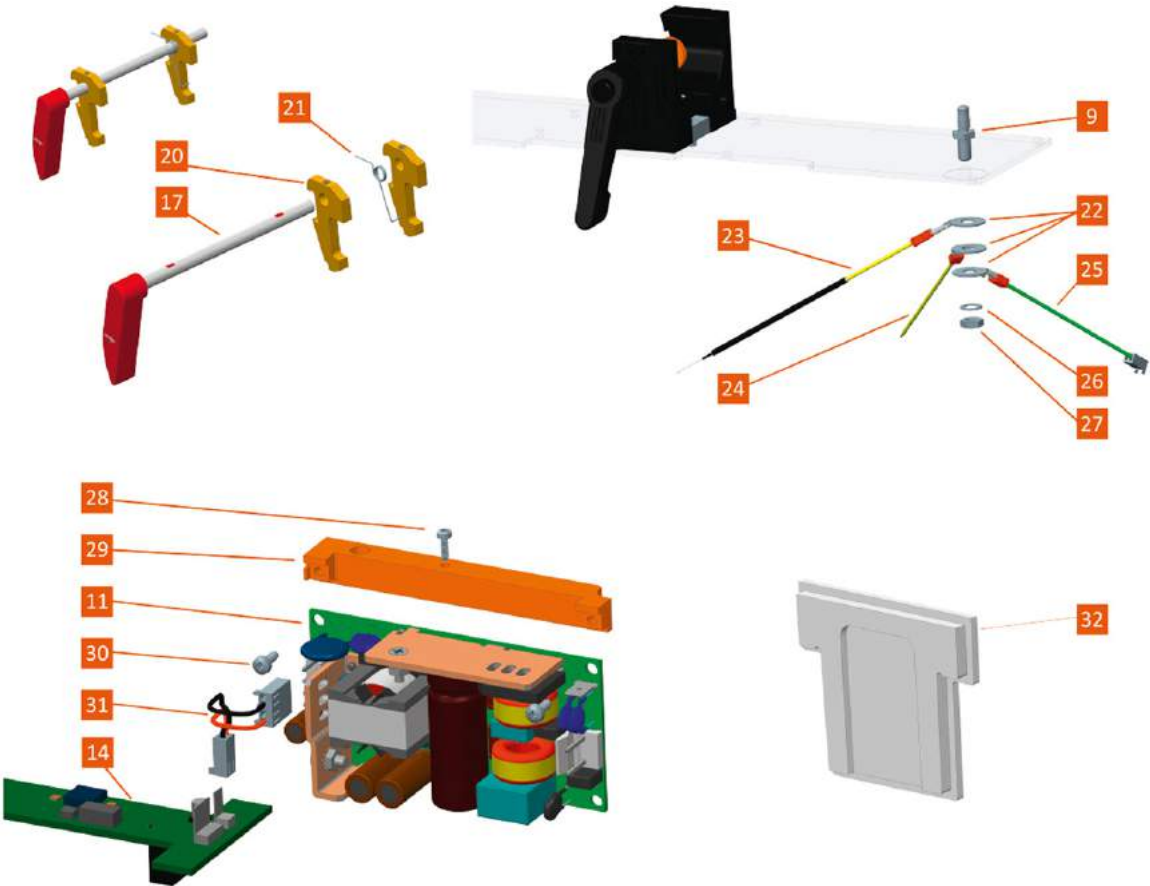
Figure 11 Exploded views - details
