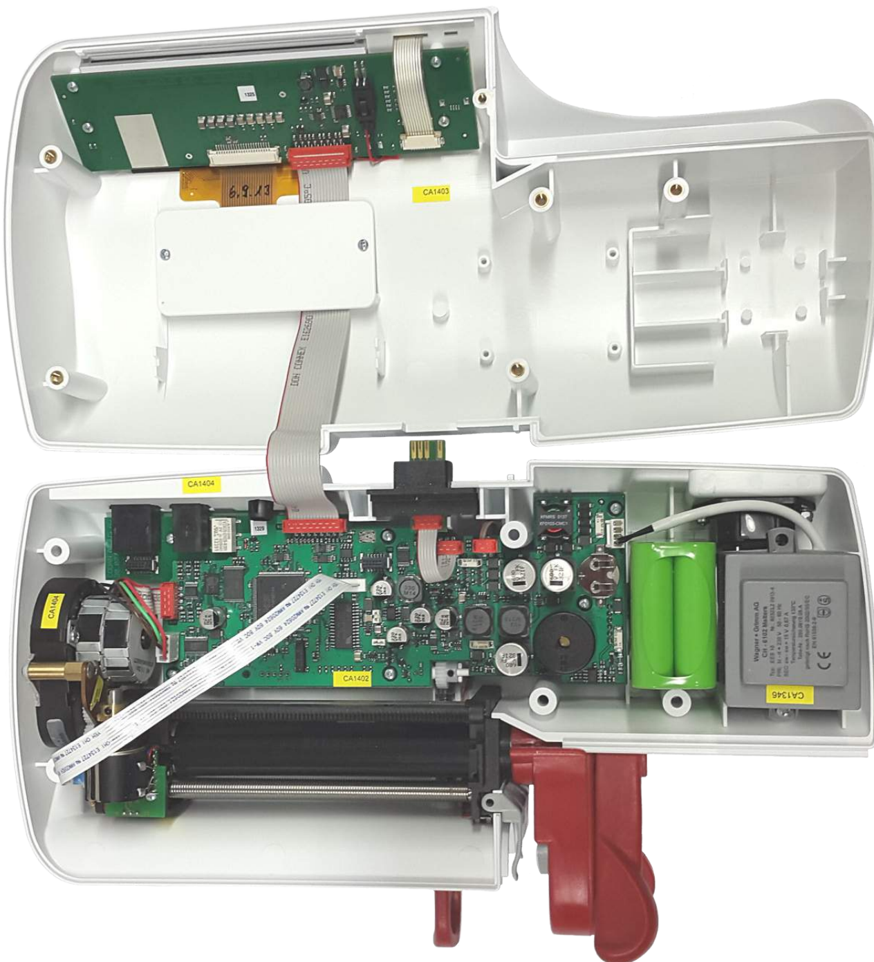
Figure 2 A606S - opened view, complete
